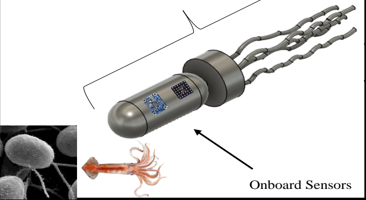
Bundled Flagellum
