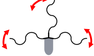
Tumble Flagellum
