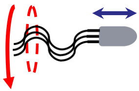
Bundled Flagellum
