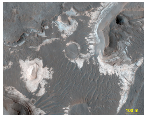
Figure 2. Example of light-toned layered deposits within Ladon Valles (unit Hl_1 ). Portion of HiRISE enhanced color image ESP_020759_1595.
