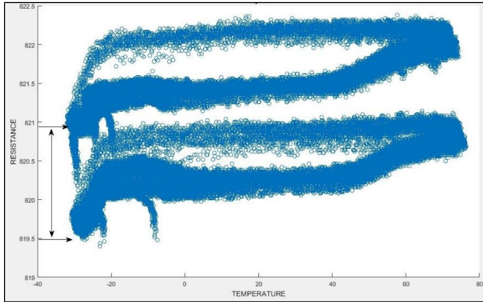
Fig. 3. Example of a resistor's response to cyclic temperature changes and an irreversible change of approximately 1.5 Ω. This change in resistance is consistent with the breaking of one grid line.
