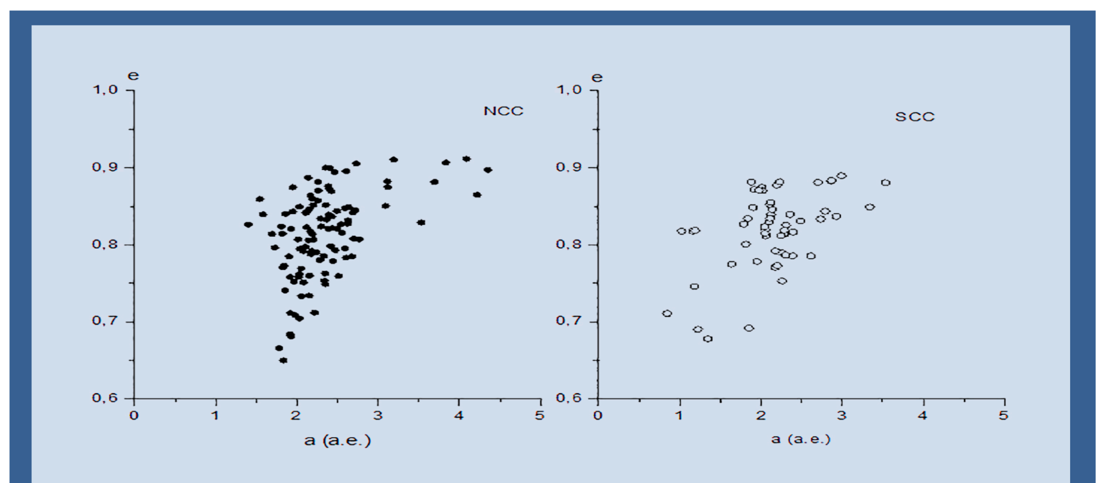
Fig.1 Changing the orbital elements (eccentricity) of the NCC branches (left), SCC (right)
