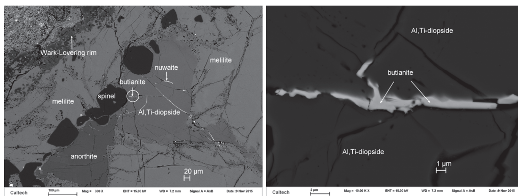
Fig. 1. Back-scatter electron images showing butianite in a crack within Al,Ti-diopside in the CAI ACM-2 .
