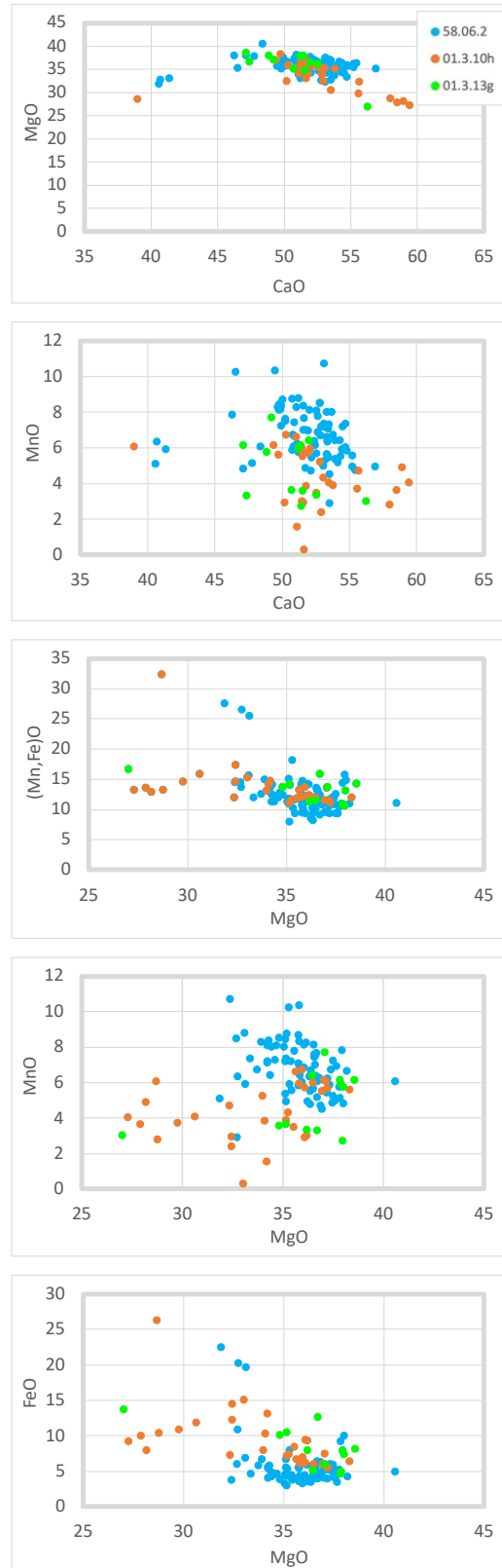
Fig. 2. Compositional correlations for dolomites in C1 materials in Kaidun expressed by their CaO, MgO, FeO, and MnO contents (mol%).
