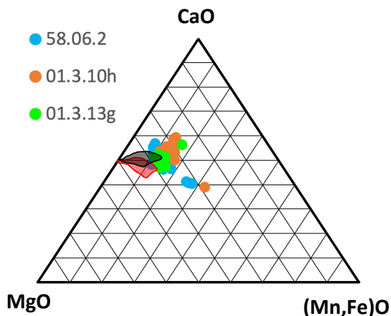
Fig. 1. Dolomite compositions of C1 materials in the Kaidun meteorite (mol%). The area circled by the red line is the compositional region of dolomites in CI chondrites and the area circled by the black line is the compositional region of CM dolomites, respectively (Data from [4]).
