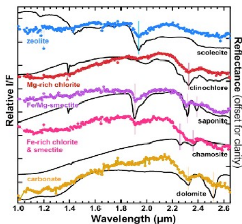
Fig. 3. Selected ratioed CRISM spectra of chlorite, chlorite/smectite, smectite, zeolite, and carbonate from our study site compared to lab spectra of minerals.
