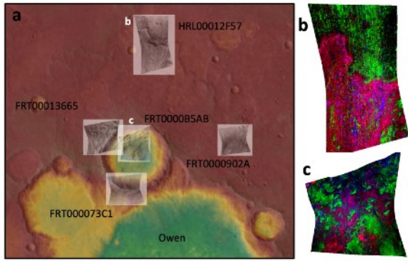
Fig. 2. A) HRSC view with CRISM IRB images. B)-C) False color mineralogy viewed in CRISM images HRL00012F57 and FRT0000B5AB with R=D2300 , G=BDI2000 , B=BD1900\_2 with pyroxene in green, chlorite in red, chlorite/smectite in pink, Fe/Mg-smectite in purple, and hydrated phases in blue.
