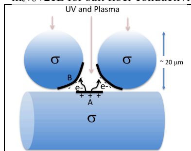
Fig 2. Illustration of differential charging on suit fibers in a weave, analogous to the differential charging with insulating regolith grains examined by [2, 3].
