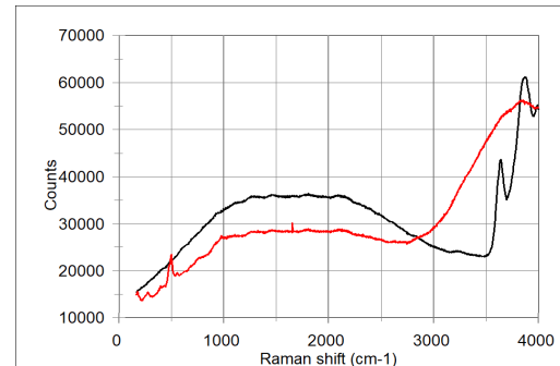
Figure 4. Raman spectra of two calcium-rich plagioclase feldspars measured at C-TAPE for the lunar-relevant spectral library. Structural and compositional variations lead to very different (and diagnostic) Raman spectra.
