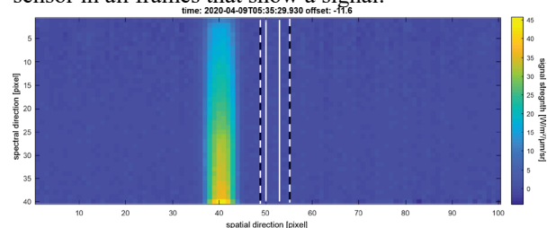
Fig. 2: Individual frame of the MERTIS instrument from the lunar observation. The vertical axis represents the spectral direction with a wavelength of \sim 13.7 \mu\text{m} on the top and \sim 7 \mu\text{m} at the bottom. The horizontal axis represents the spatial dimension with a pixel angular resolution of \sim 0.7 \text{ mrad} . Dashed vertical lines mark pixels that contain the lunar limb according to uncorrected SPICE-Kernel data. Pixel columns in and between solid vertical lines correspond to pixels that are completely contained within the lunar disk according to uncorrected SPICE-Kernel data. In the example the observed signal is offset by \sim 11.6 pixels towards smaller pixel numbers in the spatial dimension.
