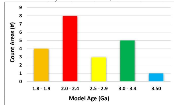
Figure 2. NE-OP lava flow eruption frequency. Two eruption peaks are observed at ~2.0 - 2.4 Ga and 3.0+ Ga.
