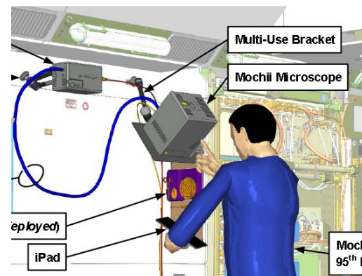
Figure 4. Mochii ISS-NL installation plan in the Japanese Experiment Module on ISS. 95 th -percentile male user shown operating Mochii using ISS-supplied iPad tablet. Sample prep kit is mounted right of Mochii on cabin bulkhead.
