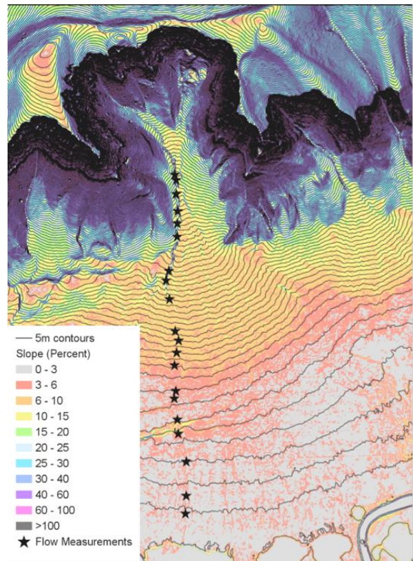
Figure 2. Slope map of the Black Mountain fan (with 5 m contours from ArcticDEM) showing our sediment transport measurement locations.
