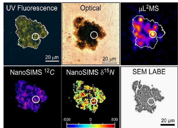
Figure 1: QUE99177 (CR3) analysis maps showing the correlation between optical and UV imaging, a mass integrated \mu\text{L}^2\text{MS} spectral map (17-250 m/z), NanoSIMS ^{12}\text{C} and \delta^{15}\text{N} isotopic images and SEM. Correlation can be achieved at the > 2\ \mu\text{m} scale. This comparative analysis was conducted on \sim 120 < 350\ \mu\text{m} of matrix per meteorite, randomly selected from whole rock.
