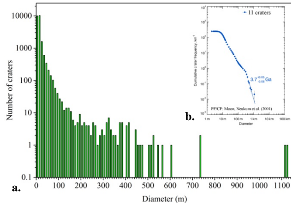
Figure 3. (a) Size-distribution of craters within the landing ellipse. The minimum and maximum diameter of craters present over the landing ellipse is \sim 2.28 m and \sim 1.13 km, respectively. (b) The inset in Figure 3a shows the crater size frequency distribution derived crater retention age of the landing ellipse.
