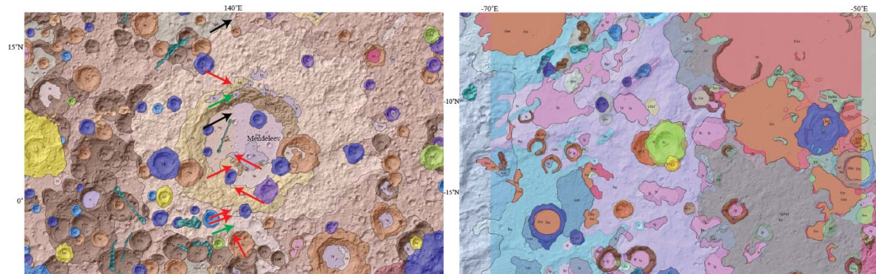
Figure 1: (Left) An example of the abutting boundary, arrows point to misaligned contacts and unit discrepancies. This is the boundary abutment between the central far side and the east side maps. (Right) An example of the overlapping boundary between the west side map and the near side map showing the discrepancies in contact placement, which will be corrected and reconciled.
