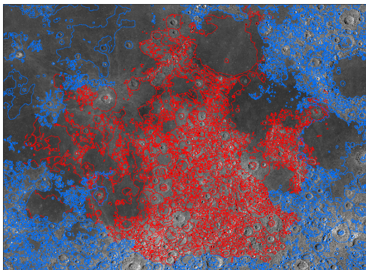
Figure 2: WAC global mosaic overlain by the contacts of the current finalized merge (blue) with the contacts from the original near side renovation that still need to be redrafted (red).
