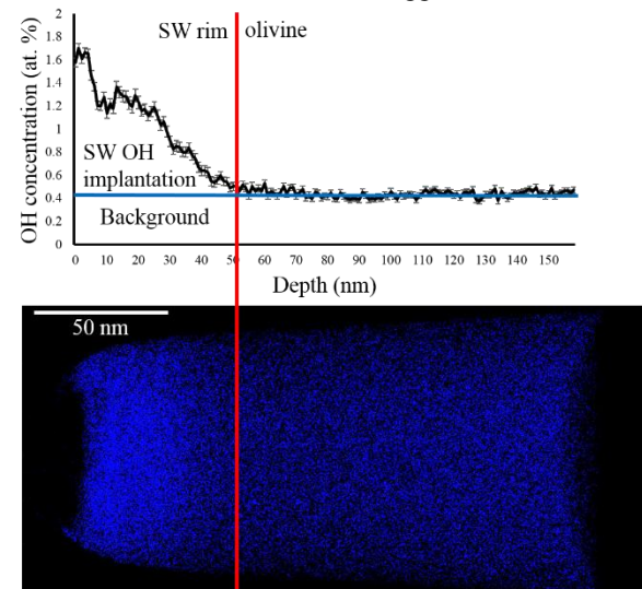
Figure 3 Atom probe specimen of a space weathered rim of Itokawa. The blue dots represent OH ions, which are enriched up to 1.6 at. % in the outer 50 nm of the particle (left hand side).
