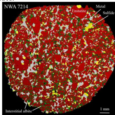
Fig. 1: X-ray map composite of NWA 7214 (Mg: Red; Fe: Grey; Na: Green; and S: Yellow).
