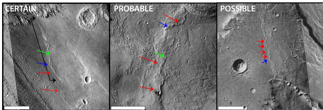
Figure 2: Examples of wrinkle ridges for each of the mapping classifications from within the study area. All scale bars are 5 km. Arrows indicate characteristics of wrinkle ridges. Black arrows indicate curvilinear map trace, blue arrows indicate ridge, green arrows indicate wrinkle, and red arrows indicate en echelon segments.
