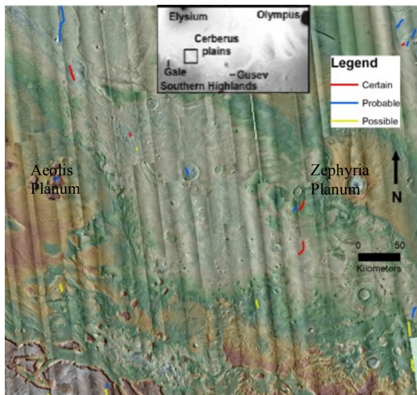
Figure 1: Currently mapped wrinkle ridges in the Aeolis Dorsa mapping area, with context map. Figure background is MOLA topography over CTX mosaic. Colored lines denote certainty categories: red denotes certain, blue denotes probable, and yellow denotes possible (see Table 1).
