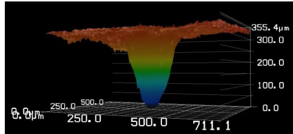
Figure 1: Ablated pit 500 pulses. 3D model made with microscope Keyence VK-100.
