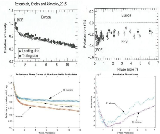
Fig. 3 Top. Rosenbush et al [9] RPC and PPC for Europa. Bottom. RPC and PPC of \text{Al}_2\text{O}_3 samples measured in this study. Europa's RPC can be explained due to a fine-grained regolith of extremely high void space.
