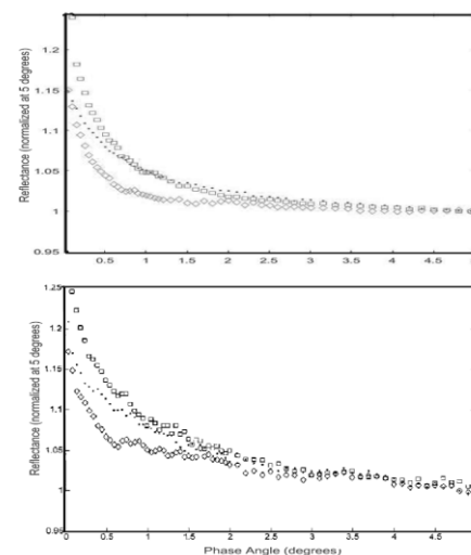
Fig. 1. Top. RPCs from this study for three particle sizes of \text{Al}_2\text{O}_3 . Diamonds – 30 \mu\text{m} , Squares – 1.0 \mu\text{m} , Dots- 1.0 \mu\text{m} . Bottom. Same as above except from [7]. These three reflectance measurements are consistent with the HRP.
