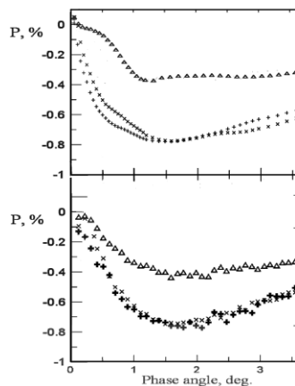
Fig 2. Top. PPCs for three particle sizes of \text{Al}_2\text{O}_3 from this study in which the samples were presented with polarized light and the intensity of the reflected component was measured. Triangles indicate 1.0 \mu\text{m} , crosses indicate 0.5 \mu\text{m} , and pluses indicate 0.1 \mu\text{m} . Bottom. PPCs of the same materials when presented with non-polarized light and the polarization of the reflected component was measured. The absence of a significant difference in these phase curves is consistent with what would be expected based on the Helmholtz reciprocity principle.
