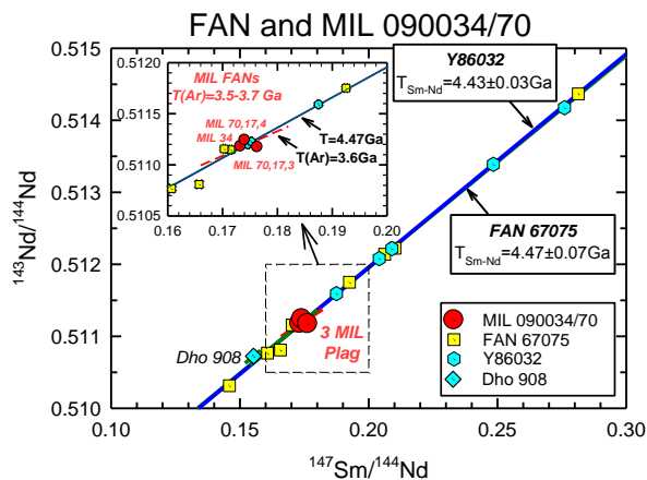
Figure 3. Sm-Nd data for density-separated plagioclase from MIL 34 and MIL 70 compared to mineral isochrons for 67075 and Yamato 86032. Bulk rock data for Dhofar 908 of the Dhofar 489 family also are shown.
