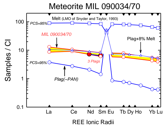
Figure 4. REE modeling of a simple petrogenesis model for the precursors of MIL 090034/70.
