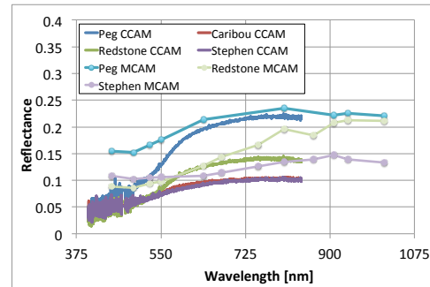
Figure 3: Chemcam passive spectra for Peg, Redstone, Caribou and Stephen with Mastcam full filter spectra for Peg, Redstone and Stephen. These targets were all found to be high in Mn with Chemcam LIBS [1,2]. Note the relatively flat, featureless spectra that are also characteristic of Mn-oxide laboratory spectra.
