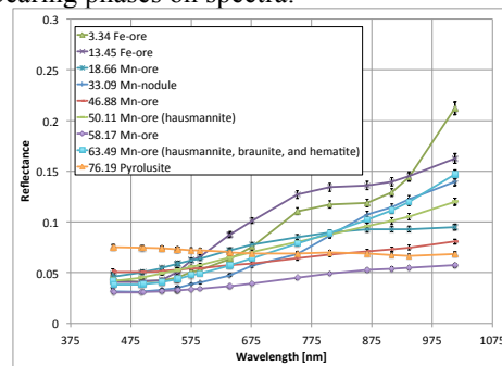
Figure 1: Laboratory visible to near infrared spectra of powdered Mn-oxide standards at p=35 degrees downsampled to Mastcam filter bandpasses. From ~500 – 900 nm the spectrum “flattens” with higher Mn-content. MnO content of samples is provided in the legend.
