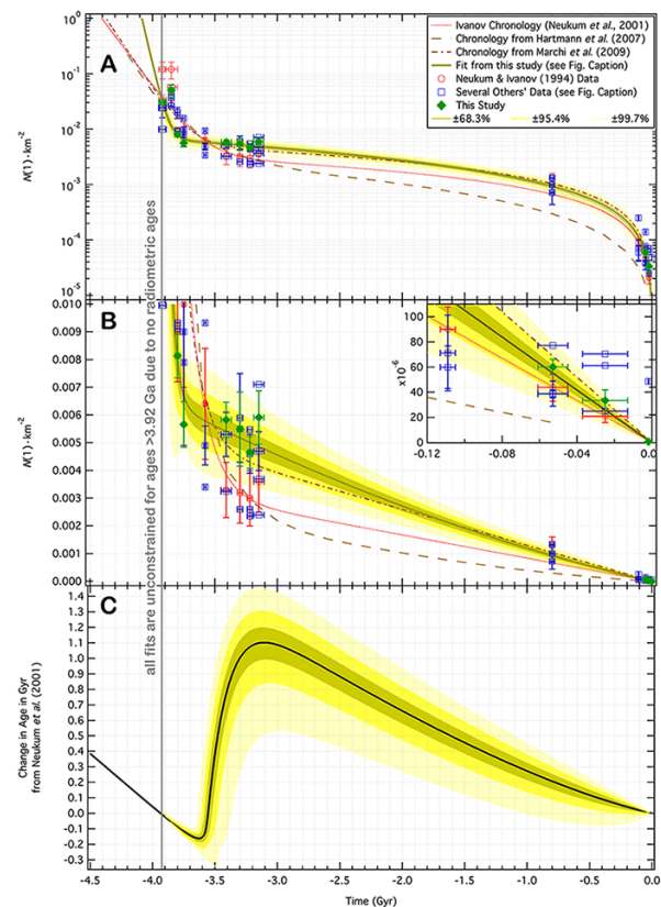
Figure 1: A and B— The canonical chronology [18] compared with revisions [13–14] and this work. Panel A shows the function on semi-log axes, while Panel B focuses on the recent cratering rate on a linear plot with the last 120 Myr inset. Data originally used by [10] are displayed with those from this study and several comparison works [3–5,8–11,14–15]. C— Difference between the new chronology and [18] as a function of age in the old chronology. 1\sigma , 2\sigma , and 3\sigma confidence bands are overlaid.
