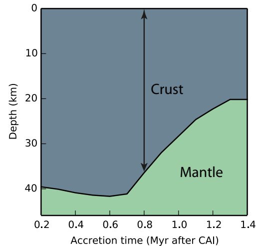
Figure 2: The crust, considered here as the less refractory material brought to the surface by melt migration is represented in grey, while the underlying olivine rich mantle residue is colored in green. Increasing the accretion time, makes the ^{26}\text{Al} energy supply decrease. This results in less melting of the mantle and in a thinner crust.
