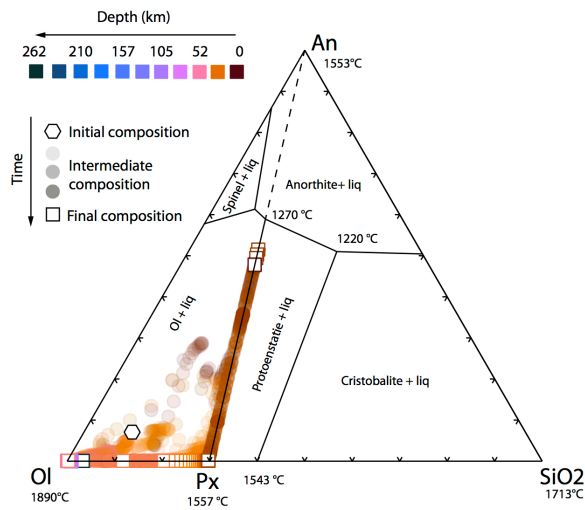
Figure 1: Olivine - Anorthite - \text{SiO}_2 system derived from [13]. Rock compositions computed in our model are overplotted, for a H type derived initial silicate composition and an accretion time 0.7 Myr after CAI formation. The initial composition is shown with a white hexagon, intermediate states are shown with filled circles, which become less transparent with time. The final state when silicate crystallization is completed is shown with white filled squares. The color of the symbols shows the depth dependency.
