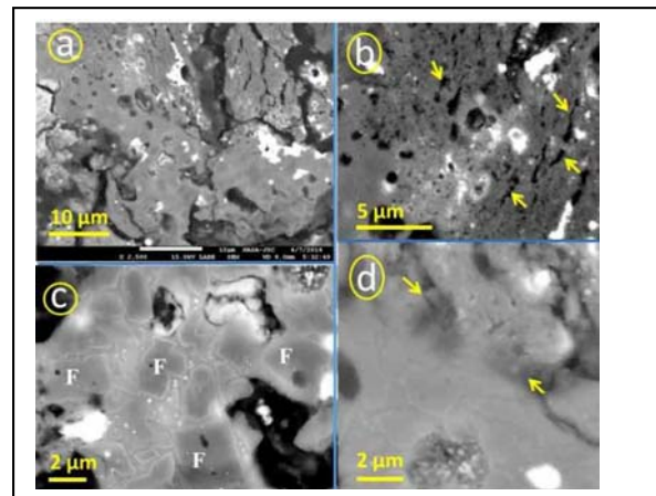
Figure 1. BSE images of a probable agglutinate in Orgueil. (a) Image of the entire agglutinate grain. (b) Close-up of partially dehydrated (heated) matrix at the edge of the agglutinate. Arrows indicate dehydration cracks in the matrix phyllosilicates. (c) Close-up of the center of the agglutinate grain, where complete melting has occurred, and cooling has produced normally-zoned olivine crystals (forsterite cores – F) in mesostasis glass. (d) Close-up of the gradation between melted and unmelted material at the agglutinate edge.
