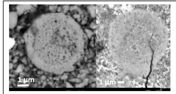
Figure 3. Beads. (left) Vesicular glassy bead from Orgueil. (right) Serpentine bead in Nogoya. Note the mottling, resembling the vesicular glassy Orgueil bead.
