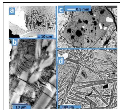
Figure 2. BSE images of shock melt vein materials in Kaidun. (a) & (b) From the CM1 lithology, serpentine faithfully pseudomorphs a vein originally consisting of zoned, acicular olivine crystals nucleating into pyroxene composition mesostasis. (c) & (d) A fragment of a vein, still fresh, consisting of acicular plagioclase ( An_{22}Ab_{76}Or_2 ) nucleating into augite mesostasis (mainly Fs_{22}Wo_{36} ). After [5].
