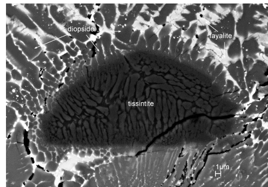
Fig. 5. Enlarged BSE image of Fig. 4 of fine-grained tissintite with surrounding diopside and fayalite.
