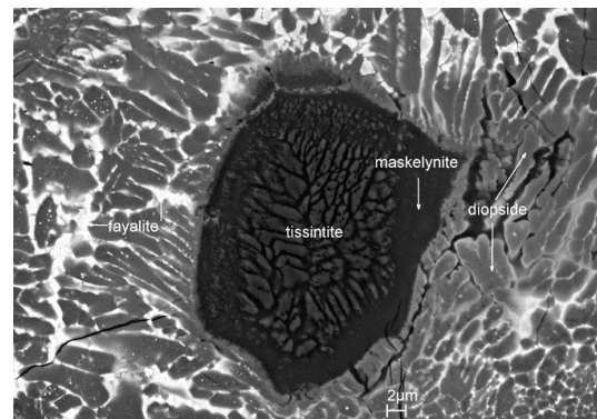
Fig. 6. BSE image showing tissintite crystals within Msk with surrounding diopside and fayalite in a melt pocket in Tissint section UT1.
