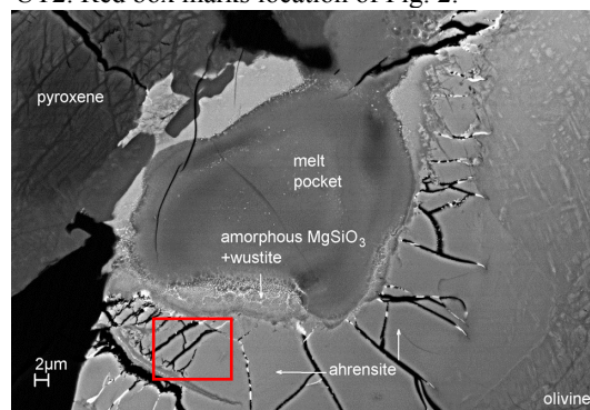
Fig. 2. Enlarged BSE image of Fig. 1, revealing ahrensite domains with surrounding phases. Red box marks location of Fig. 3.
