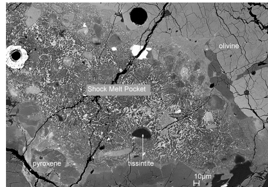
Fig. 4. BSE image showing tissintite in a shock melt pocket in Tissint section UT2.
