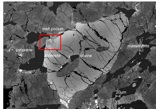
Fig. 1. Back-scatter electron (BSE) image showing ahrensite and shock melt pocket in Tissint section UT2. Red box marks location of Fig. 2.
