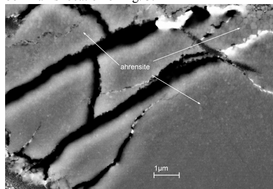
Fig. 3. BSE image of a portion of Fig. 2, revealing submicrometer- to nanometer-sized polycrystalline ahrensite.
