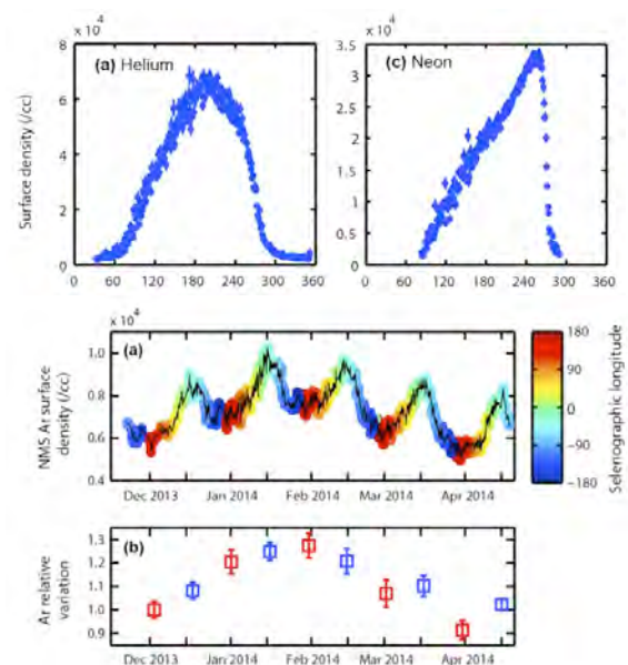
Fig. 2. (top) LADEE NMS results for 4 He and 20 Ne. Horizontal axis is solar longitude, with 0 at noon, 90 at sunset, 180 at midnight and 270 dawn. (bottom) Time variations in 40 Ar over the LADEE mission. Argon density maximizes over the western maria. From [7].
