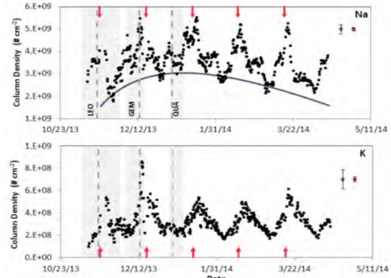
Fig. 4. LADEE UVS Na and K column densities (40 km grazing altitude) during the mission. Red arrows denote Full Moon, when the Moon is in the geomagnetic tail.
