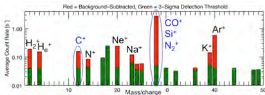
Fig. 3. Exospheric species identified by their pickup ions. Because of the very significant carbon detection, mass 28 is likely at least partly \text{CO} . From [8].
