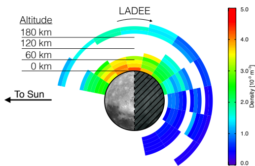
Fig. 1. LDEX dust density variation with local time and altitude. From [5].
