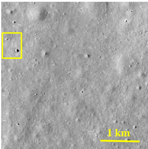
Figure 2. 15 km 2 area of the eastern Taurus Littrow pyroclastic deposit, within region of interest (LROC NAC image; area of Figure 3 outlined)
