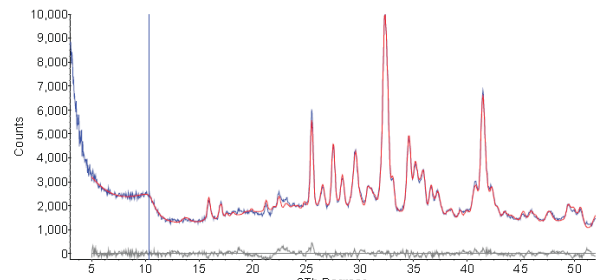
Figure 2: 1D XRD pattern of John Klein with observed (blue) versus calculated (red) patterns, and difference curve at the bottom (gray). Vertical line marks the smectite 001 diffraction maximum at \sim 10^\circ .
