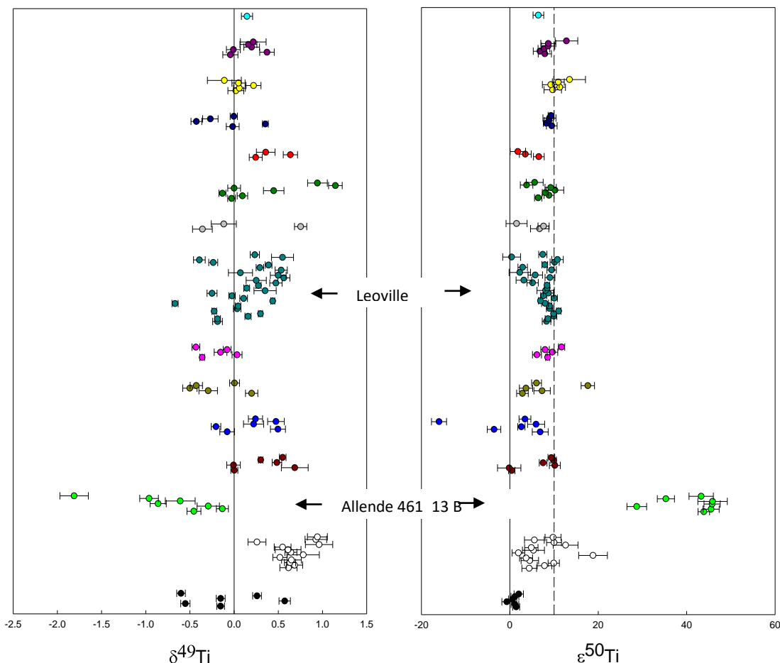
Figure 1. (a) LA-MC-ICPMS \delta^{49}\text{Ti} data for a suite of CAIs from Allende, Efremovka, Leoville, and NWA 2364. (b) LA-MC-ICPMS \epsilon^{50}\text{Ti} data for the same suite of CAIs.
