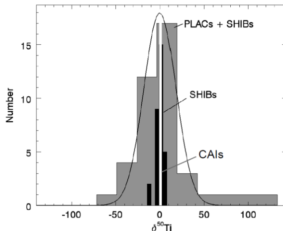
Figure 2. \delta^{50}\text{Ti} ( \epsilon^{50}\text{Ti}/10 ) data for hibonite grains from Liu (2008). The average CAI value is plotted with a white line at \epsilon^{50}\text{Ti} = 10 ( \delta^{50}\text{Ti} = 1 ).
