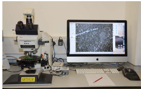
Figure 1: Rotating stage microscope with Mindstorm motor
